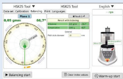
One-Plane Balancing
