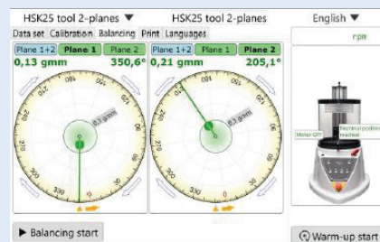
Two-Plane Balancing
